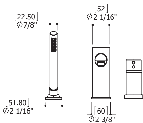
mixing valve
