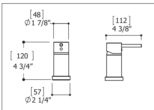
mixing valve
