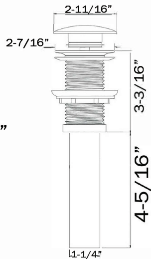
DRAIN VIEW
