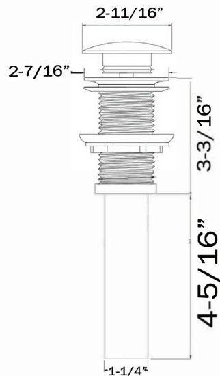
DRAIN VIEW
