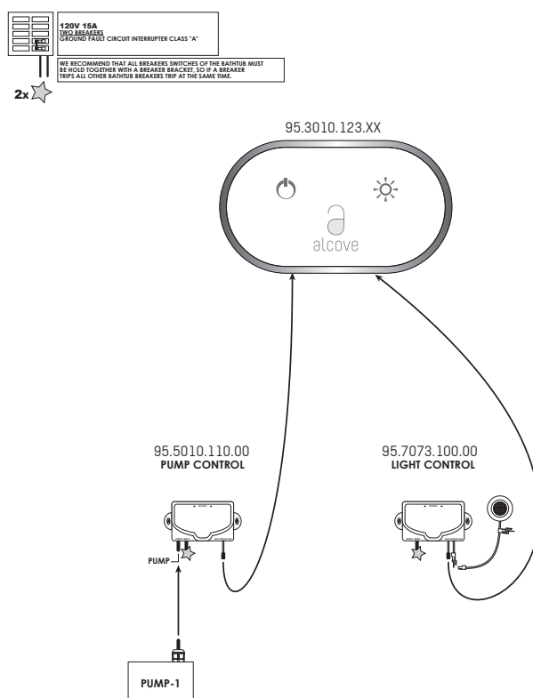
Fig. 22 Whirlpool and Chromotherapy light
