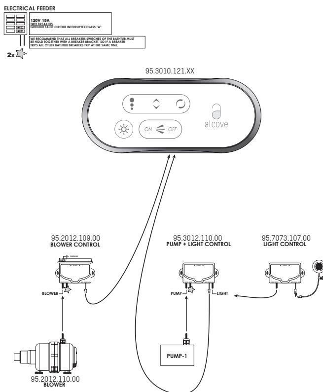
Fig. 26 Combined Whirlpool and Balne-Air or Vibro-Air and Chromotherapy Light
