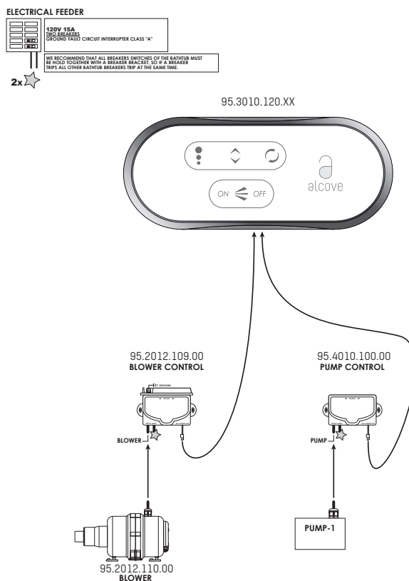
Fig. 25 Combined Whirlpool and Balne-Air or Vibro-Air
