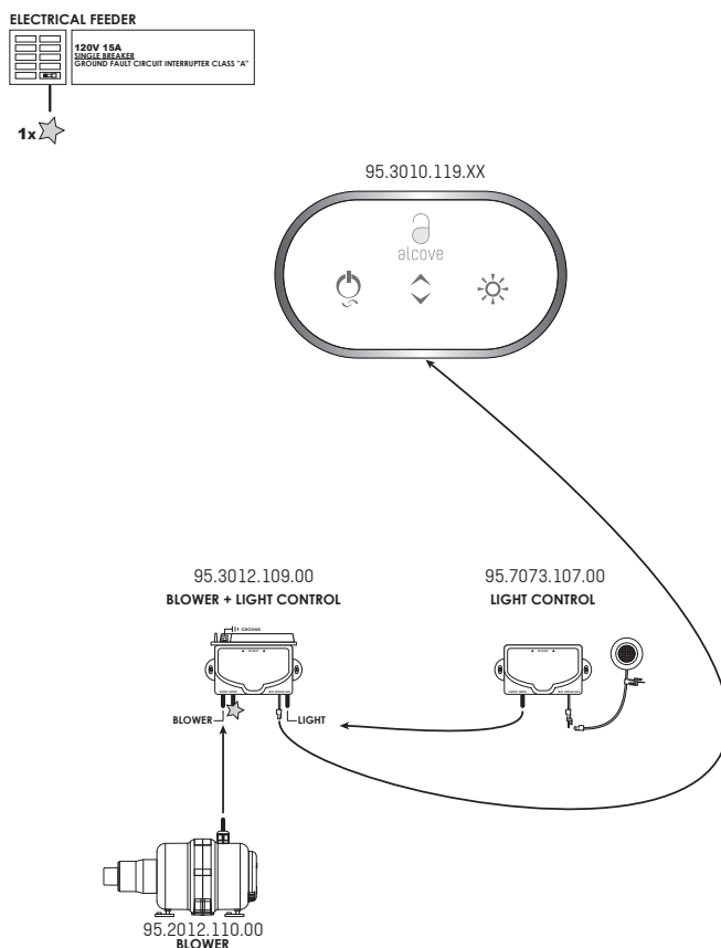
Fig. 24 Balne-Air or Vibro-Air and Chromotherapy light
