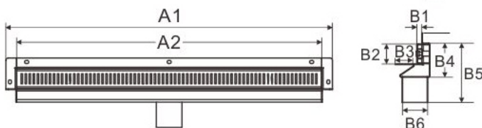
Grate and Gutter rough-in drawing
