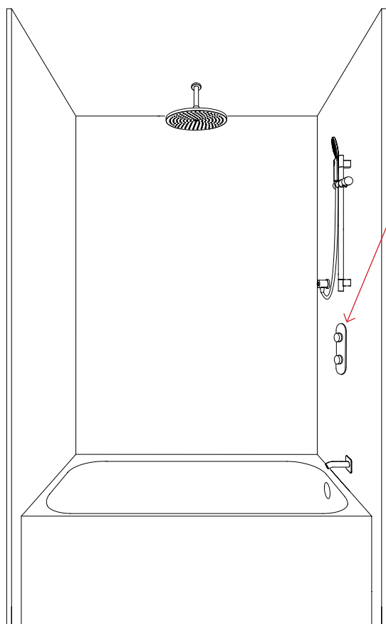
4" CEILING ARM, RAIL & TUB SPOUT BRAS DE PLAFOND DE 4", RAIL ET BEC DE BAIN
