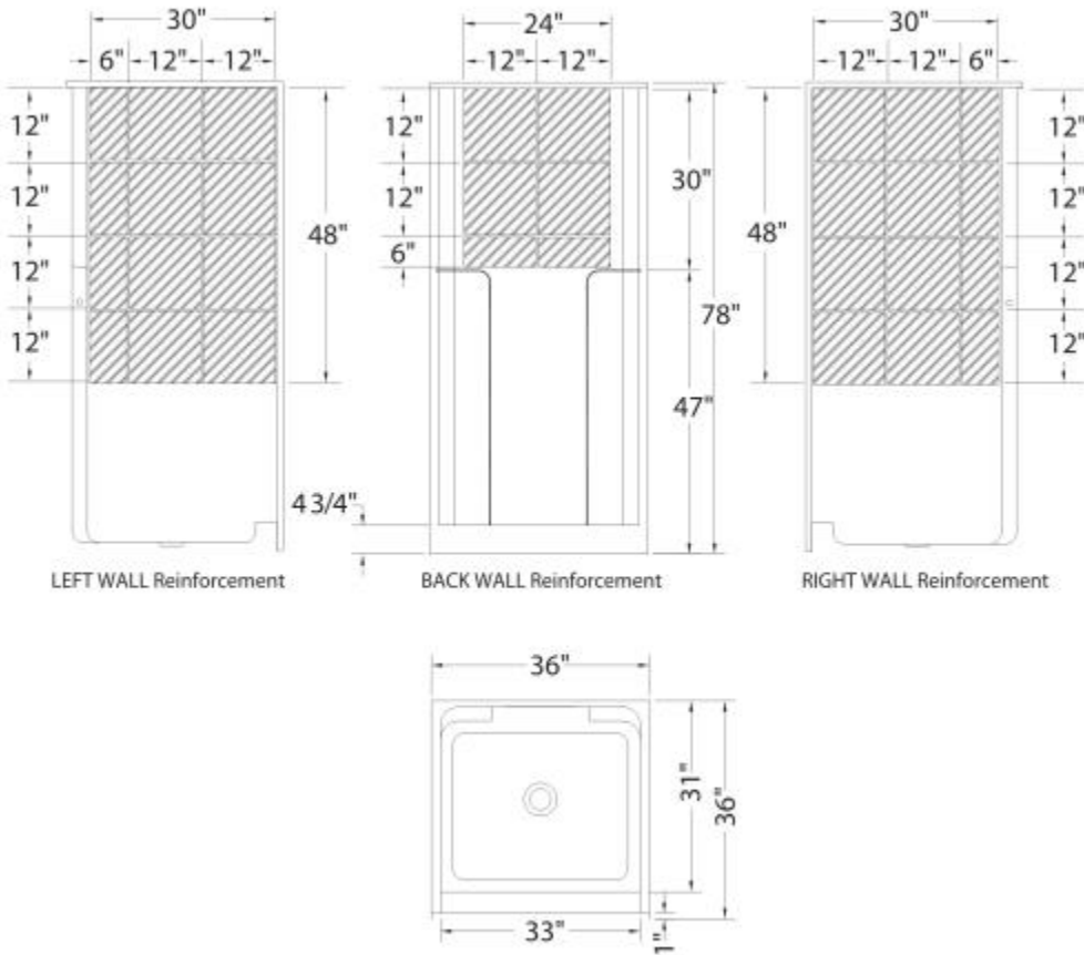
Full Wall Reinforcement Shown
