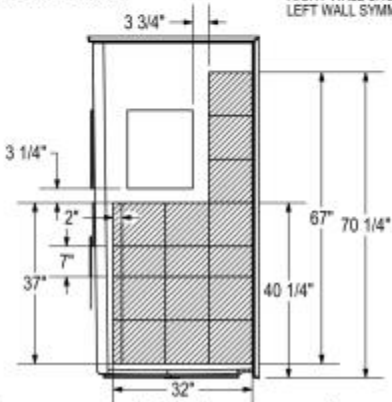
REINFORCEMENT BACKING
